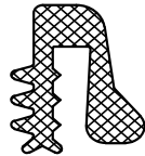
Profile for 2 mm made of: EPDM conductive
